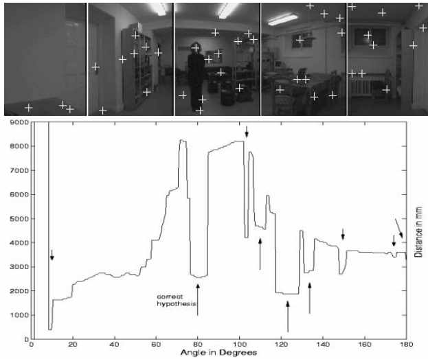
Fig. 7. Generating hypotheses separately from laser and vision data.
