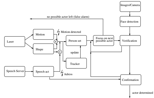
Fig. 6. Schematic overview of detecting the user.
